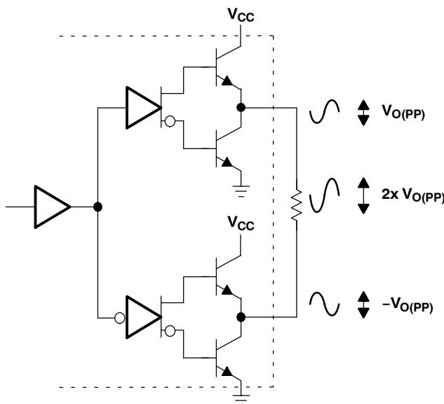
Figure 24. Bridge-Tied-Load Configuration
