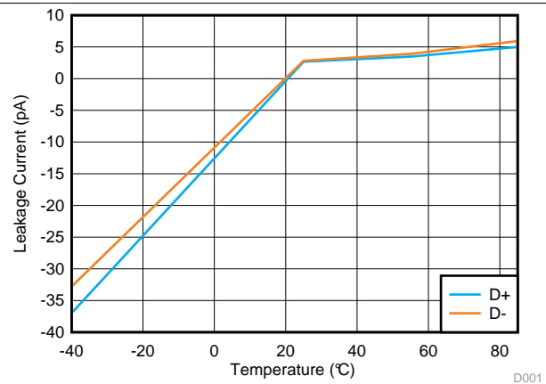
Figure 2. Leakage Current vs Temperature ( V_{IO} = 2.5\text{ V} )
