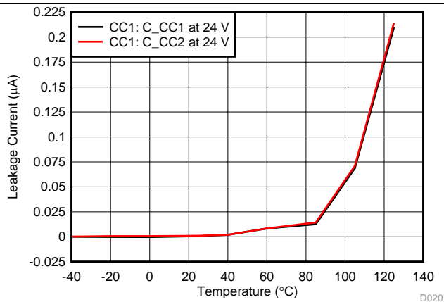
Figure 13. CC OVP Leakage Current vs Ambient Temperature at C_CC = 24 V
