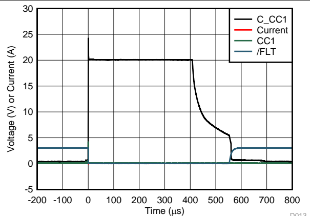
Figure 2. CC Short-to-VBUS 20-V VM = 3.3 V
