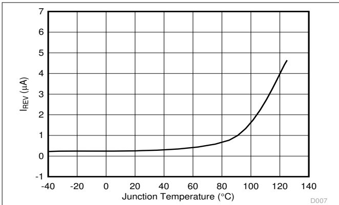
Figure 6-5. Reverse Leakage Current ( I_{REV} ) vs Temperature
