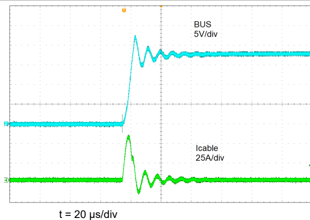
Figure 9-6. DC-DC VIN Floating, BUS Shorted to Battery
