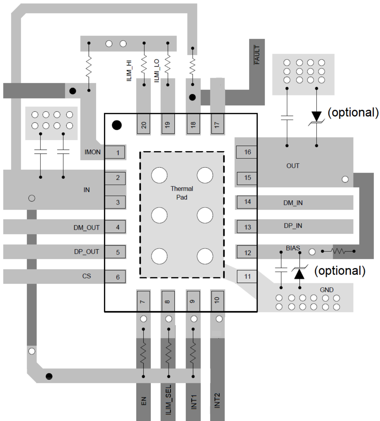
Figure 9-11. TPD3S713x-Q1 Layout Diagram
