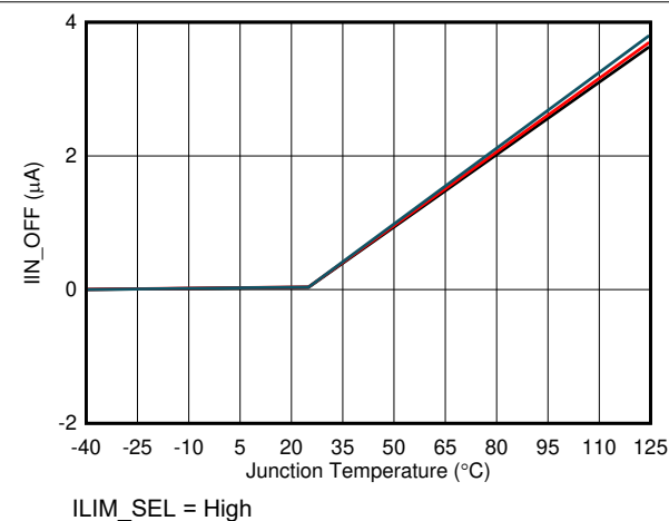
Figure 6-6. Disabled IN Supply Current vs Temperature
