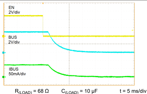
Figure 6-17. Turn-off Response
