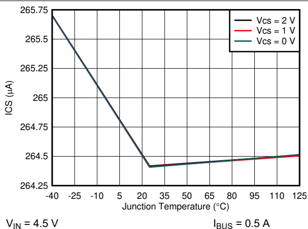
Figure 6-13. I_{(IMON)} vs V_{(CS)} Voltage
