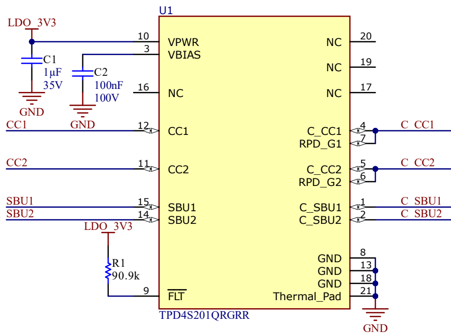
Figure 7-2. TPD4S201-Q1 Dead Battery
