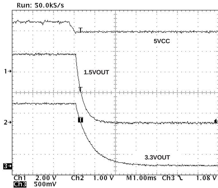
Figure 4. Power-Down Sequence
