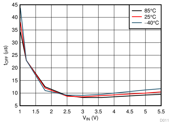
Figure 6-33. Turn-Off Time
