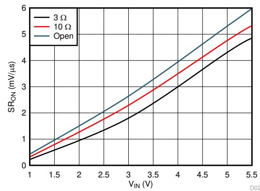
C_L = 100 \mu F TPS22916C TPS22916CN TPS22916CL Figure 6-32. Slow Slew Rate vs Load Resistance
