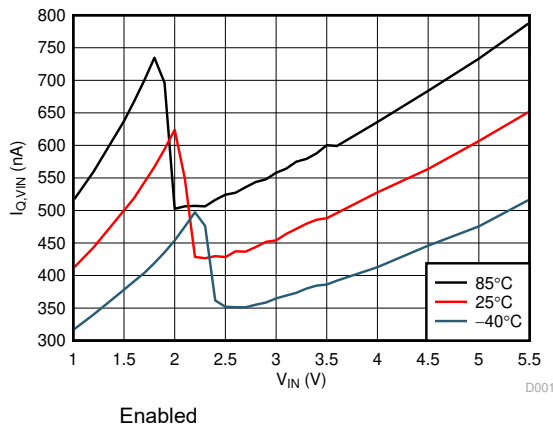
Figure 6-5. Quiescent Current
