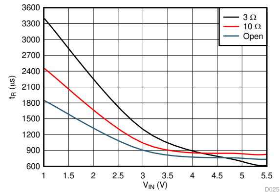
C_L = 100 \mu F TPS22916C TPS22916CN TPS22916CL Figure 6-30. Slow Rise Time vs Load Resistance
