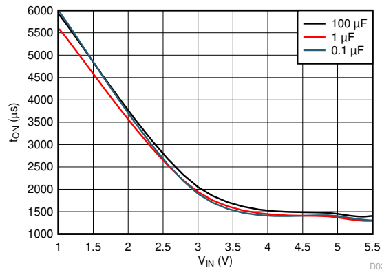
R_L = 10 \Omega TPS22916C TPS22916CN TPS22916CL Figure 6-27. Slow Turn-On vs Load Capacitance
