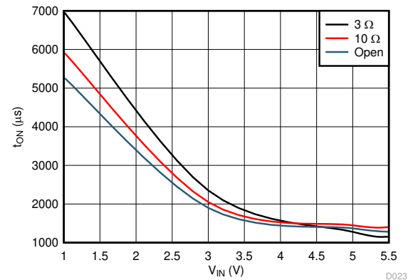
C_L = 100 \mu F TPS22916C TPS22916CN TPS22916CL Figure 6-28. Slow Turn-On vs Load Resistance
