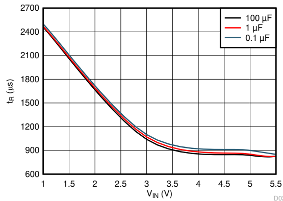
R_L = 10 \Omega TPS22916C TPS22916CN TPS22916CL Figure 6-29. Slow Rise Time vs Load Capacitance
