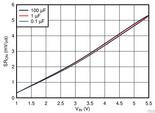
R_L = 10 \Omega TPS22916C TPS22916CN TPS22916CL Figure 6-31. Slow Slew Rate vs Load Capacitance
