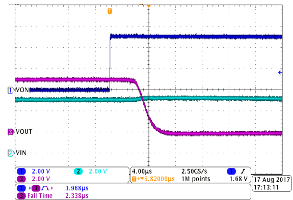
Figure 6-34. Turn-Off at 5 V (Active Low)
