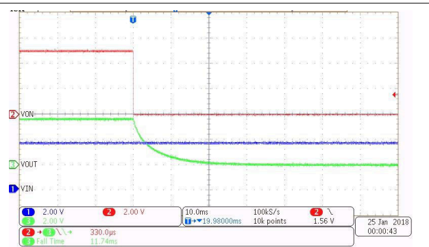
Figure 7-26. Turn-Off at 3.6 V (Open Load)
