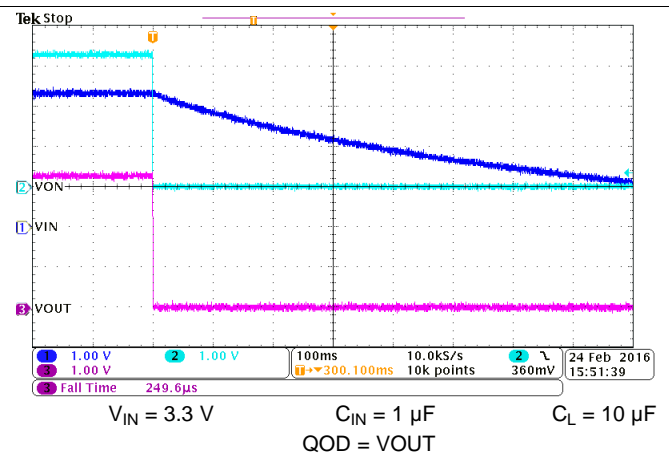
Figure 27. Fall Time ( t_F ) at V_{IN} = 3.3 V
