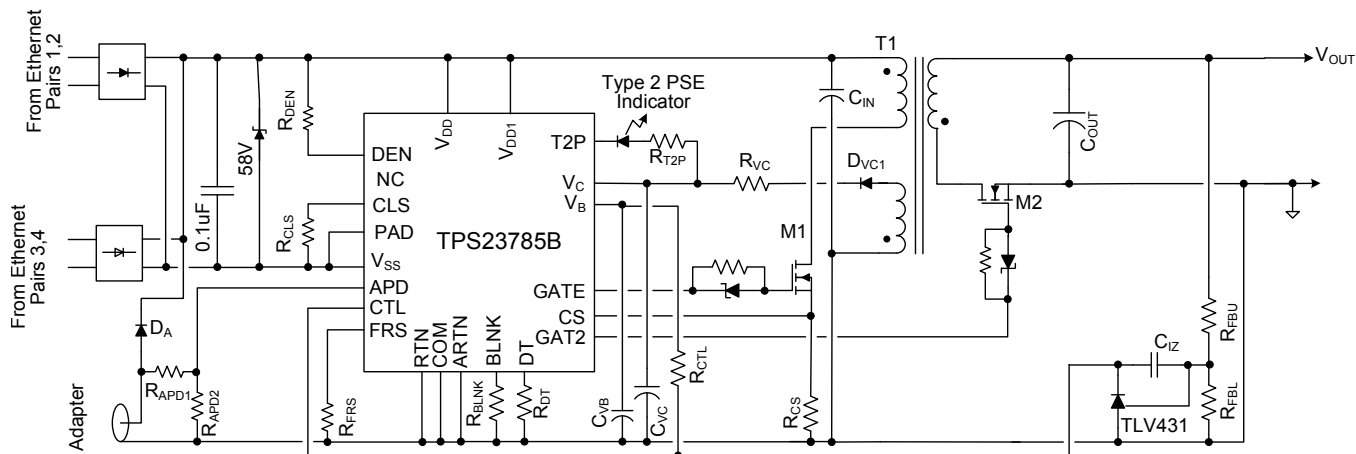
Typical Application Diagram
