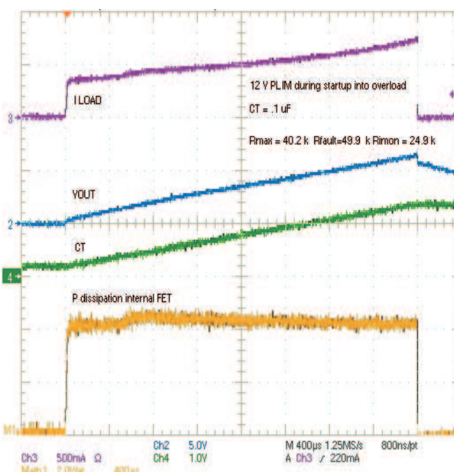
Figure 14. Power Dissipation During 12-V Startup into a 15-Ω, 140-μF Load
