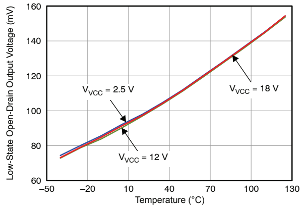
Figure 17. PGb Open-Drain Output Voltage in Low State
