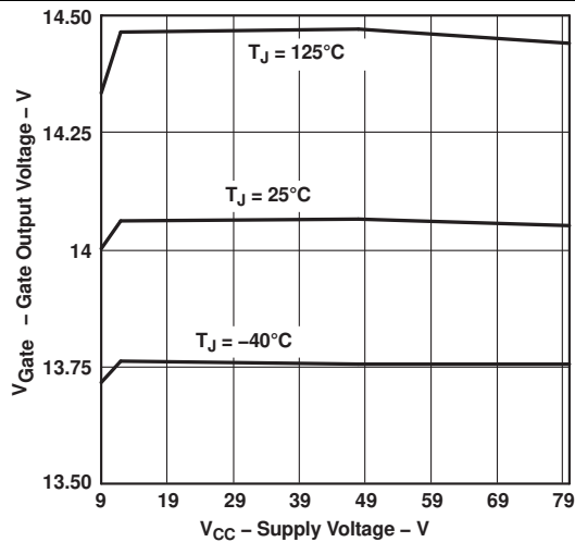
Figure 7. Gate Output Voltage vs Supply Voltage
