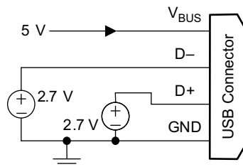
Figure 8-9. Divider 3 Mode
