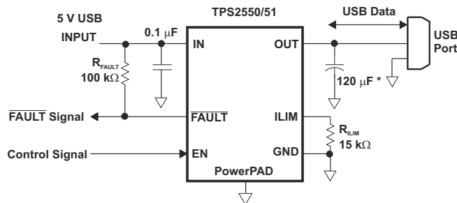
Figure 10-5. Typical Application as USB Power Switch
