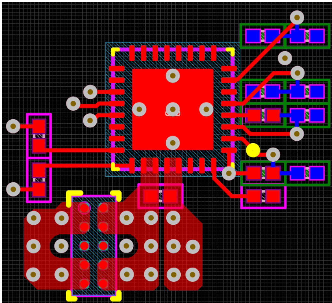
Figure 9-27. VIN_3V3, LDO_3V3, and LDO_1V5 Routing
