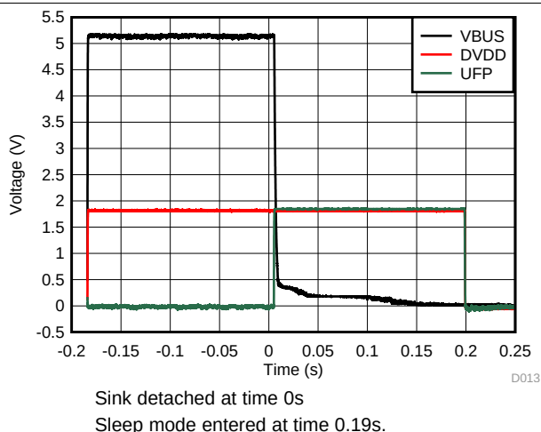
Figure 20. DVDD and \overline{ENSR} Upon Sink Attachment
