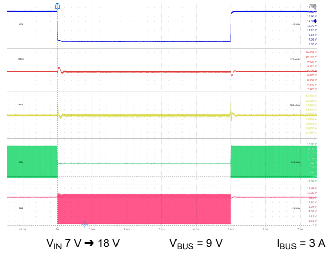
Figure 9-37. Line Transient: V_{BUS} = 9 V
