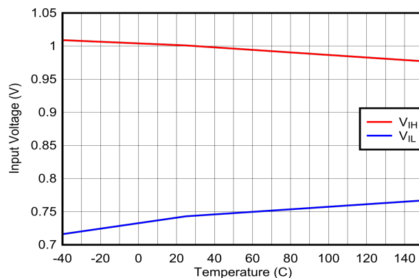
Figure 6-48. GPIO: Input Voltage Thresholds vs Temperature
