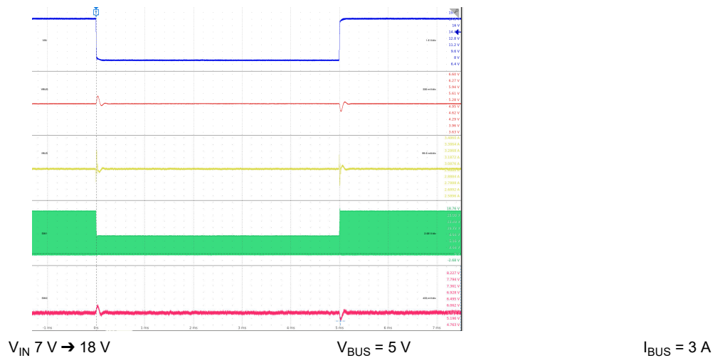
Figure 9-38. Line Transient: V_{BUS} = 5 V
