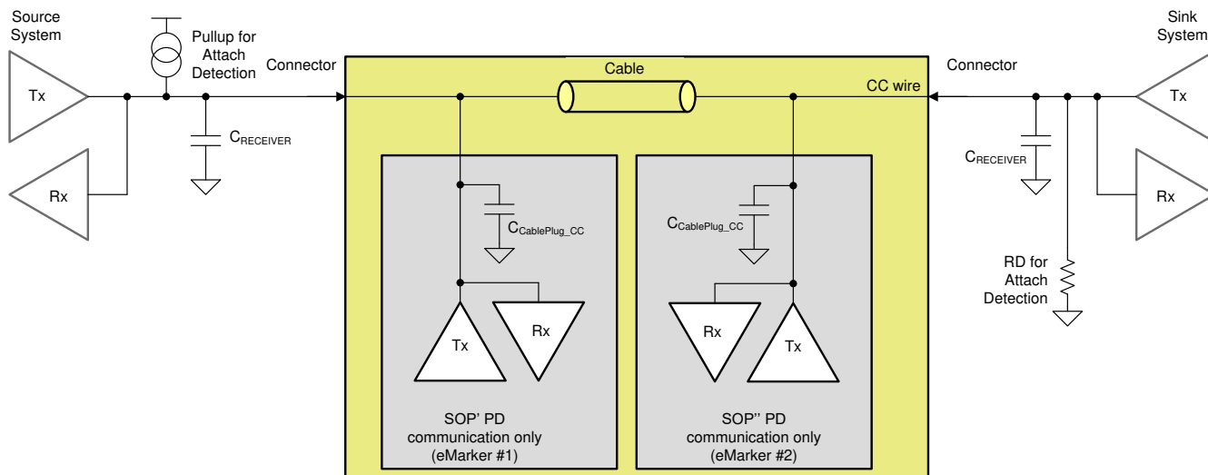
Figure 8-25. Example USB-PD Multi-Drop Configuration
