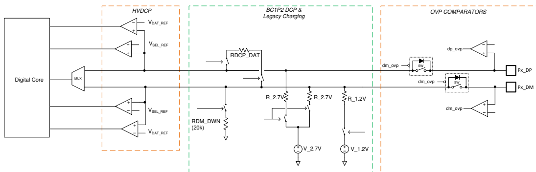
Figure 8-32. BC1P2 Functional Diagram
