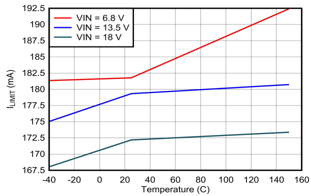
Figure 6-9. LDO_5V Current Limit vs V_{IN} and Temperature
