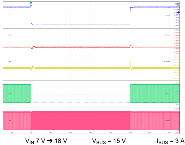
Figure 9-36. Line Transient: V_{BUS} = 15 V
