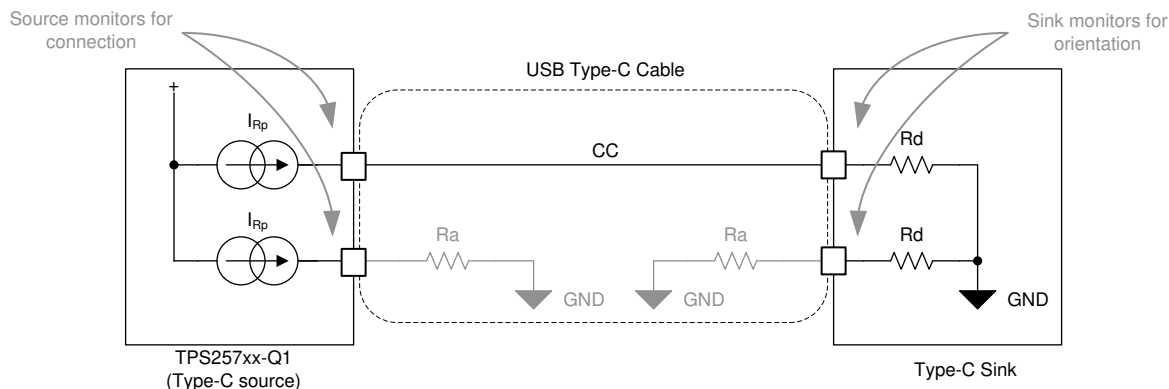
Figure 8-28. Type-C Cable
