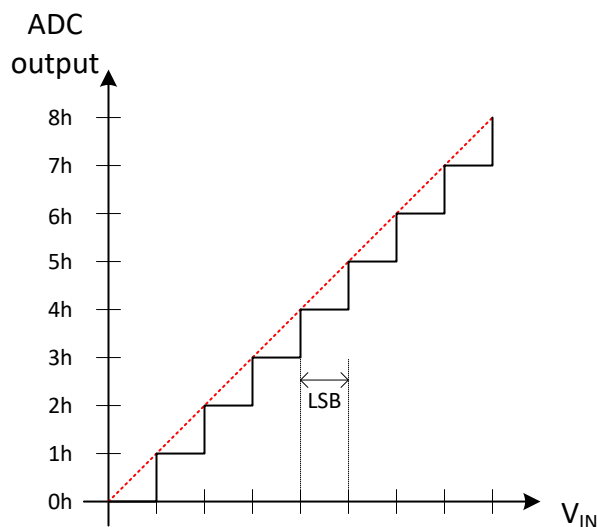
Figure 8-31. ADC Conversion
