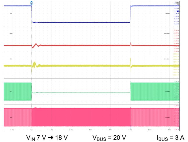
Figure 9-35. Line Transient: V_{BUS} = 20 V
