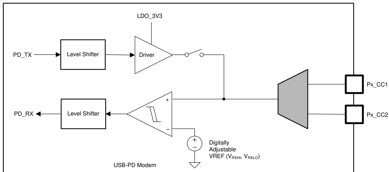
Figure 8-22. USB-PD BMC TX/Rx Block Diagram
