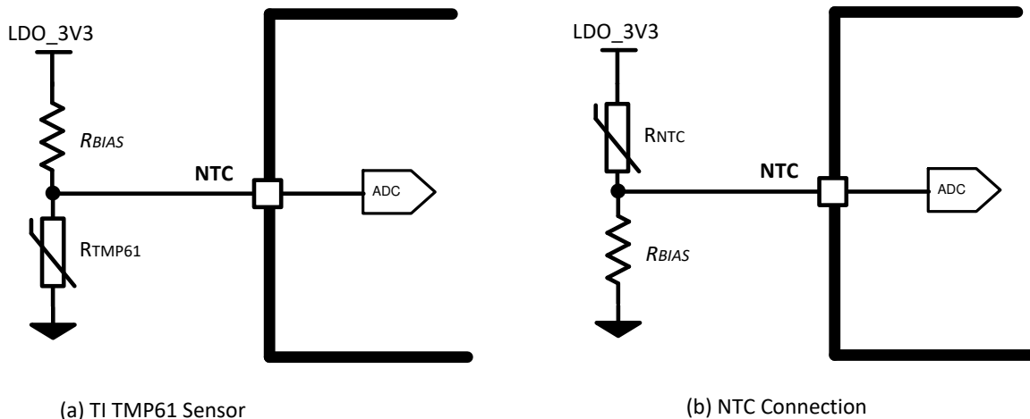
Figure 8-42. Thermistor Connections (a) PTC, (b) NTC
