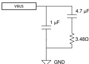
Figure 9-2. VBUS Snubber
