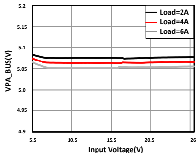
Figure 11-12. Dropout Characteristic
