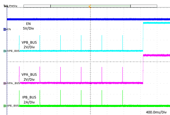
Figure 11-23. 1- \Omega Load Recovery
