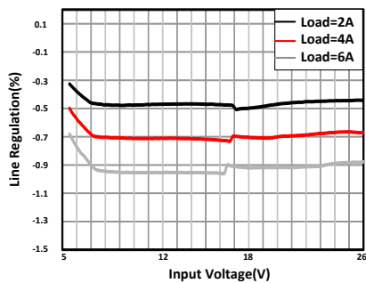
Figure 11-6. Line Regulation
