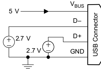
Figure 10-12. Divider 3 Mode
