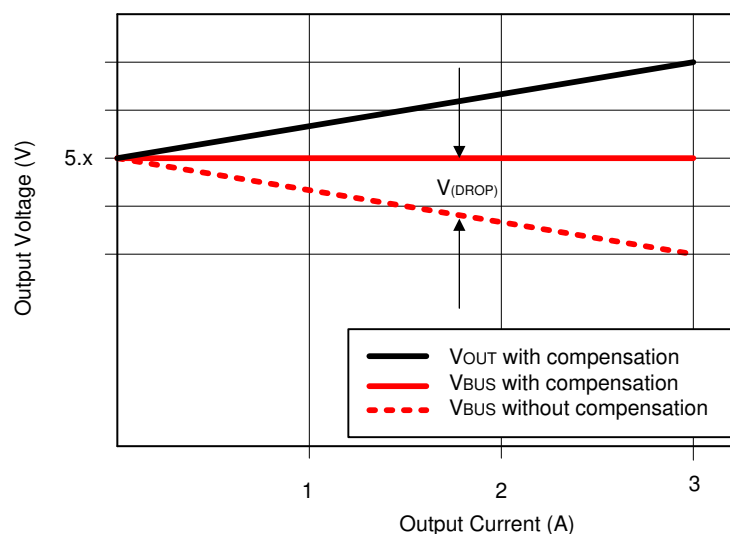
Figure 10-8. Voltage Drop
