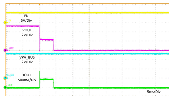
Figure 11-25. OUT short to 5.1- \Omega Load
