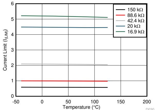
Figure 7-18. Current Limit vs Temperature Across R_{(ILIM)}
