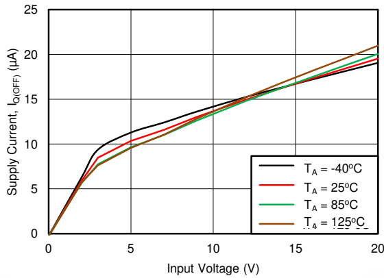
Figure 7-3. Input Supply Current vs Supply Voltage at Shutdown
