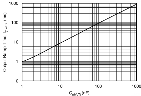
Figure 7-15. Output Ramp Time vs C_{(dVdT)}
