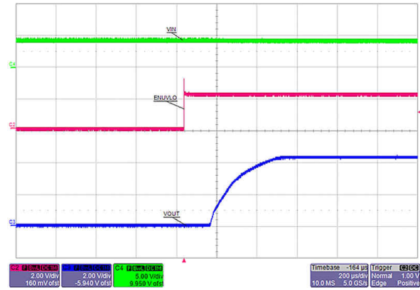
Figure 7-32. Turn ON with Enable
