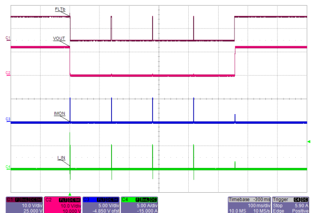
Figure 10-14. Hot Short: Auto-Retry and Recovery from Short Circuit - TPS25940-Q1
