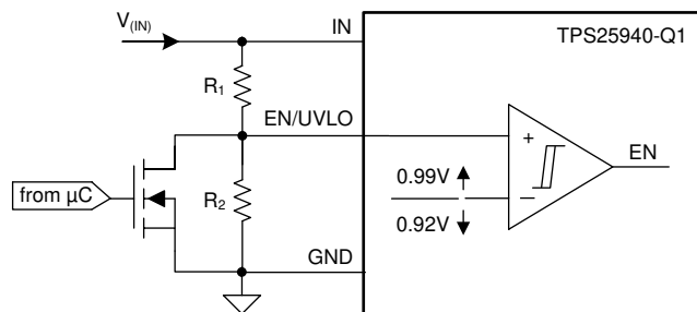
Figure 9-8. Shutdown Control
