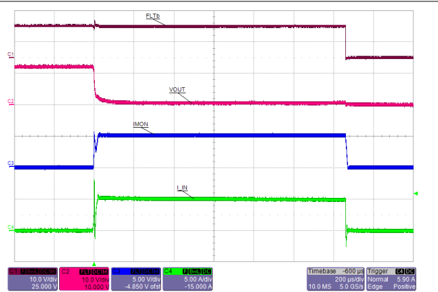
Figure 10-18. Hot Short: Latched - TPS25940L-Q1
