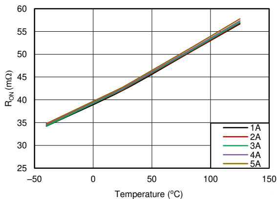
Figure 7-27. R_{ON} vs Temperature Across Load Current
