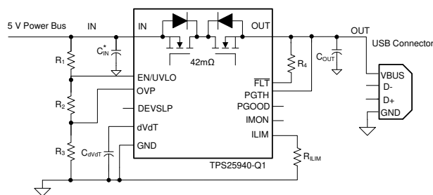
Simplified Schematic
