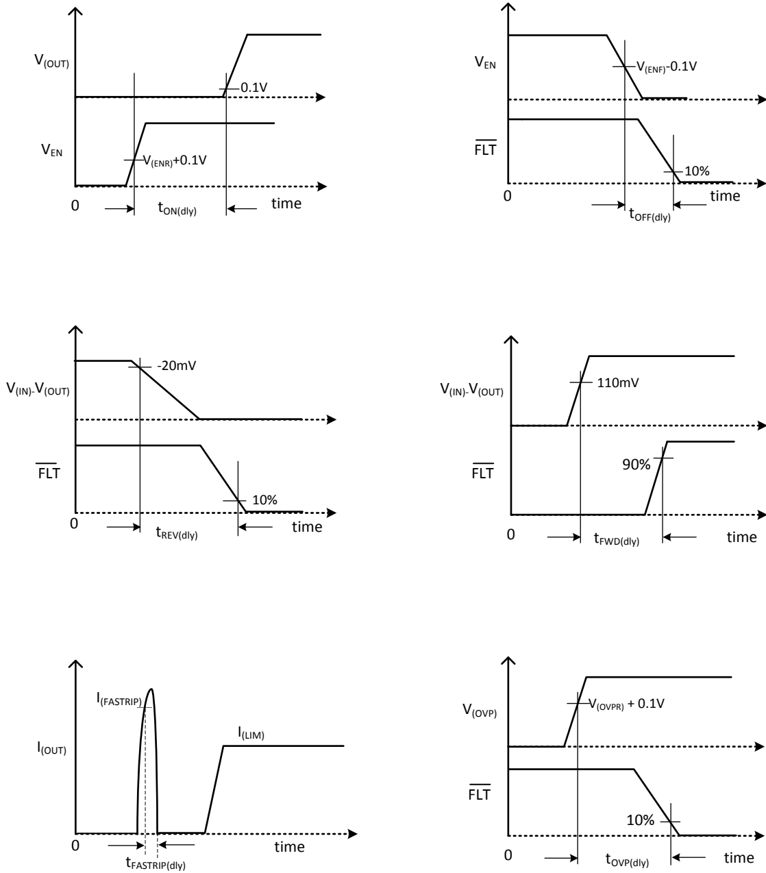
Figure 8-1. Timing Diagrams
