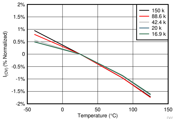
Figure 7-19. Current Limit (% Normalized) vs R_{(LIMIT)} Resistor
