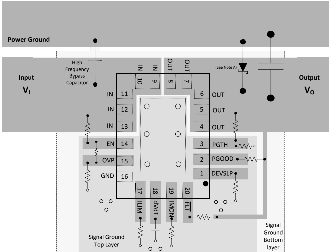
Figure 12-1. Board Layout
