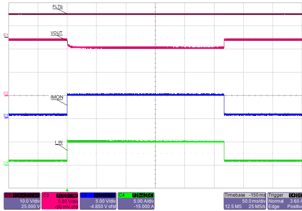
Figure 10-11. Over Load: Step Change in Load from 12 \Omega to 2 \Omega and Back
