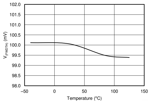
Figure 7-30. V_{(FWDTH)} vs Temperature
