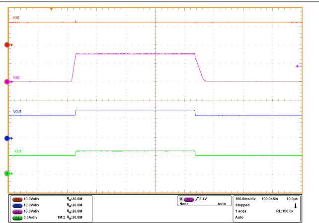
Figure 8-15. Active ORing Response
