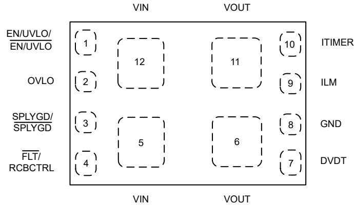
Figure 5-1. YWP Package, 12-Ball PWCSOP (Top View)
