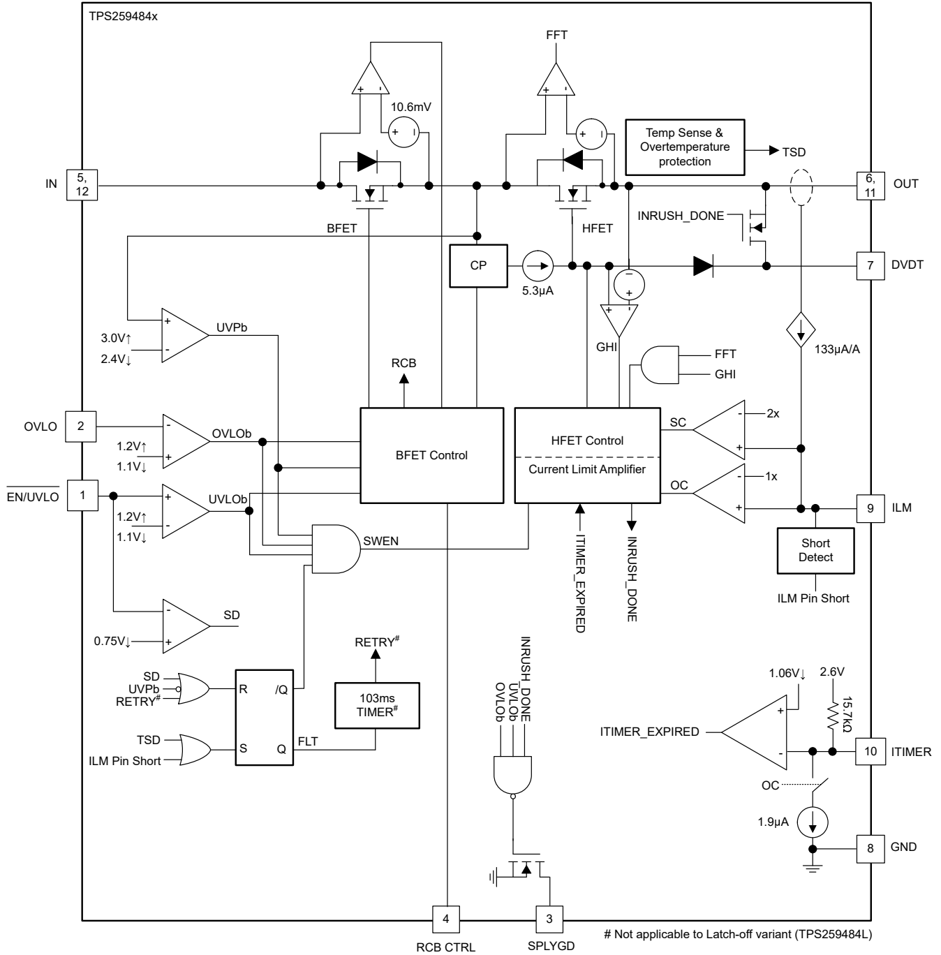
Figure 7-4. TPS25948 Block Diagram
