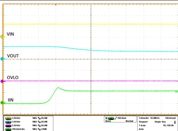
Figure 8-12. Overcurrent Protection
