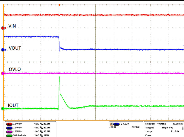
Figure 8-13. Short at Output Protection
