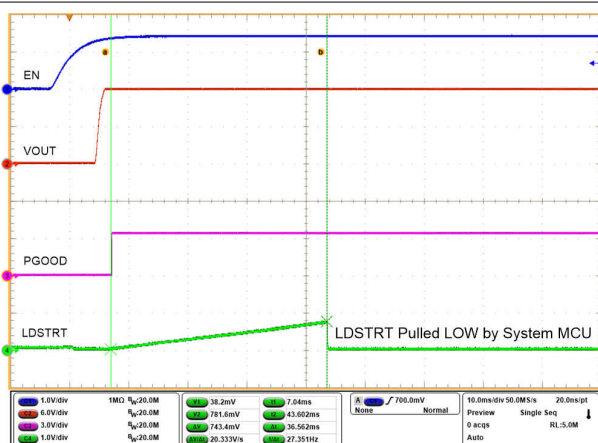
Figure 9-11. Successful Load Handshake (LDSTRT)
