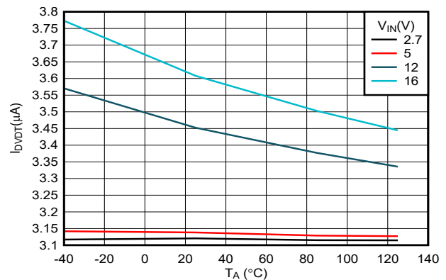
Figure 6-21. DVDOT Charging Current vs Temperature
