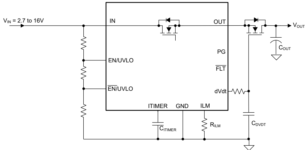
Figure 7-8. Reverse Current Blocking Using External FET
