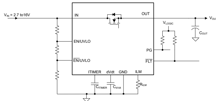
Figure 8-1. Single Device, Self-Controlled
