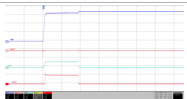
Figure 8-15. Power Up with Short Circuit on Output
