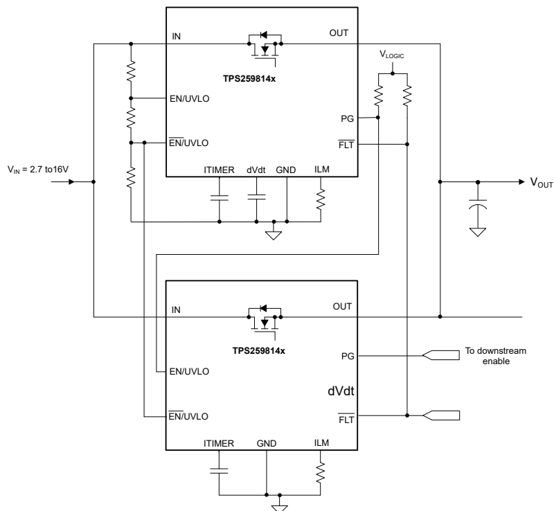
Figure 8-2. Two TPS259814x Devices Connected in Parallel for Higher Steady-State Current Capability
