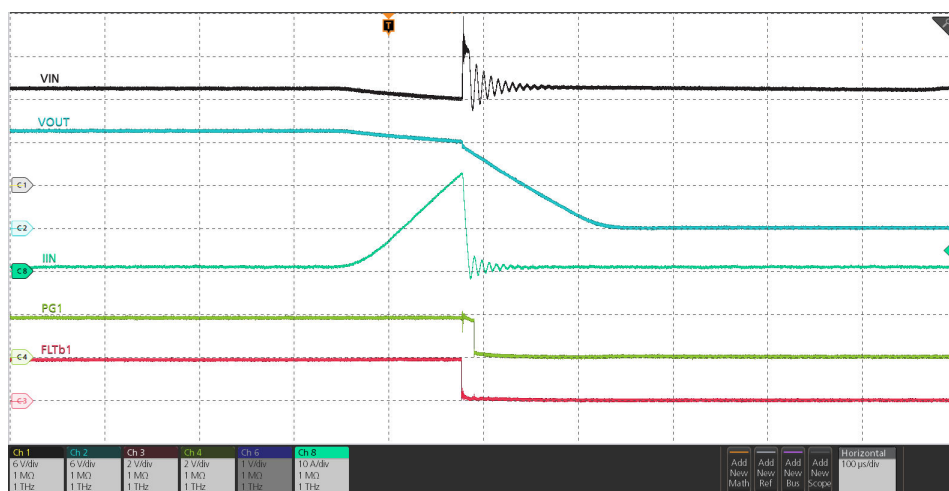
Figure 8-5. Parallel Devices Overcurrent Response
