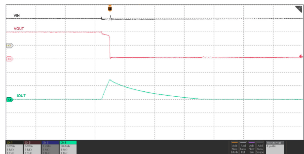
Figure 6-35. Circuit-Breaker Response
