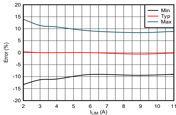
Figure 6-14. Overcurrent Threshold Accuracy (Across Process, Voltage and Temperature)
