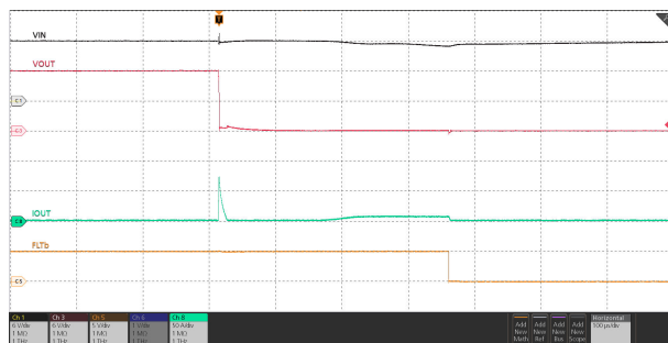
Figure 6-34. Transient Overcurrent Blanking Timer Response
