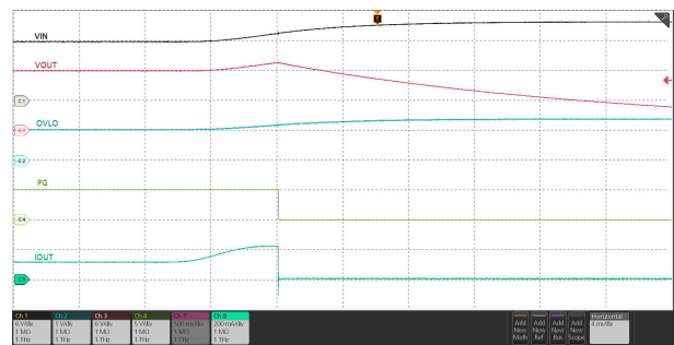
Figure 6-33. Overvoltage Lockout Response
