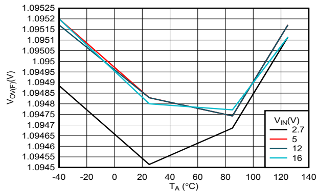
Figure 6-12. OVLO Falling Threshold vs Temperature
