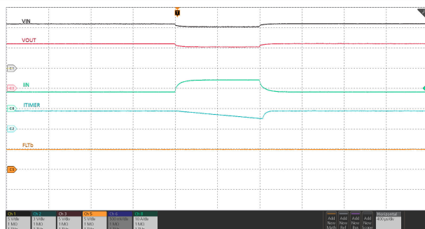
Figure 6-32. Inrush Current with Resistive and Capacitive Load
