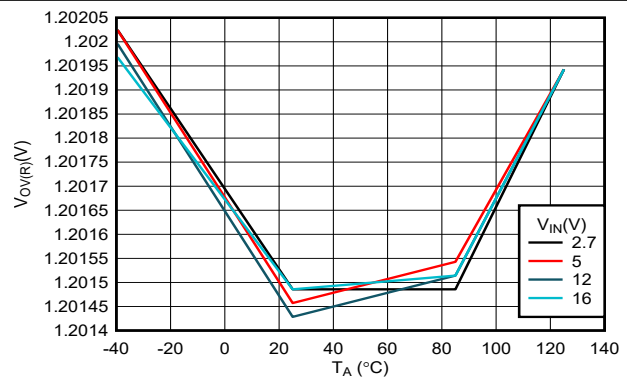
Figure 6-11. OVLO Rising Threshold vs Temperature
