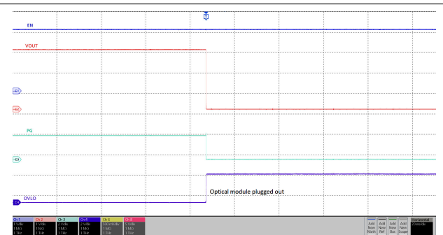
Figure 8-11. Output Voltage Profile When Optical Module is Plugged Out
