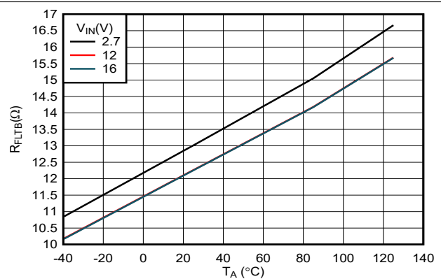
Figure 6-23. FLT Pin Pulldown Resistance vs Temperature
