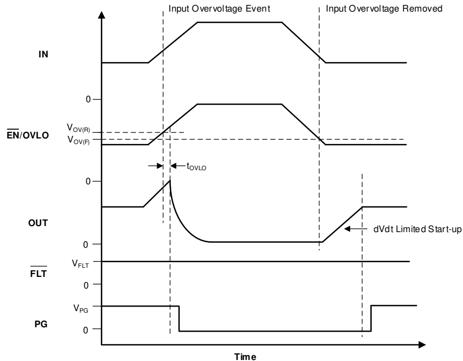
Figure 7-3. TPS25981x Overvoltage Lockout and Recovery
