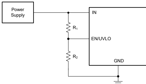
Figure 7-1. Adjustable Undervoltage Protection
