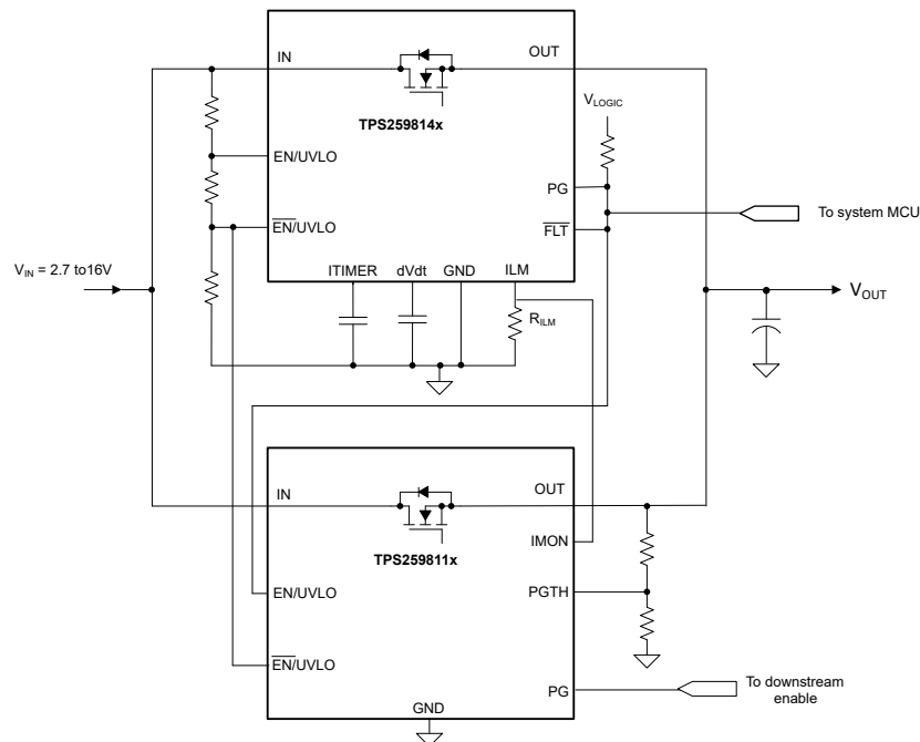
Figure 8-6. TPS259814x and TPS22811x Connected in Parallel for Higher Steady-State Current Capability
