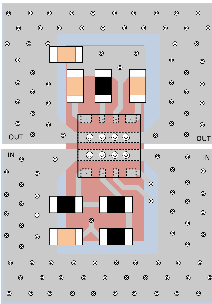
Figure 8-17. Layout Example
