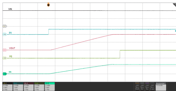
Figure 6-32. Inrush Current with Resistive and Capacitive Load
