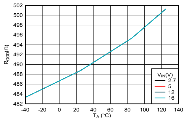
Figure 6-25. Quick Output Discharge Resistance vs Temperature
