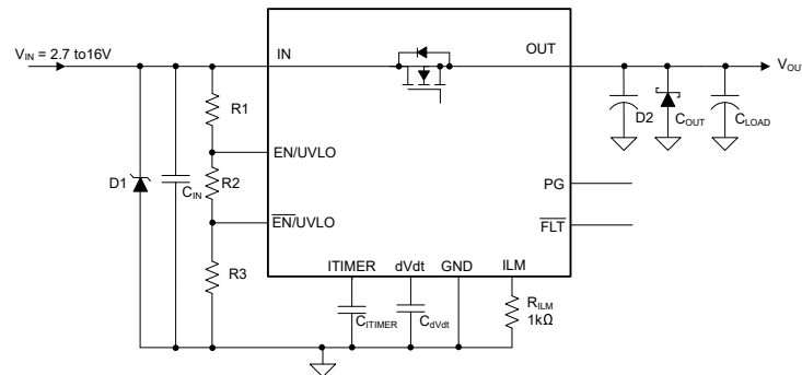
Figure 8-16. Circuit Implementation with Optional Protection Components
