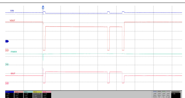
Figure 8-13. Overload Response and Recovery
