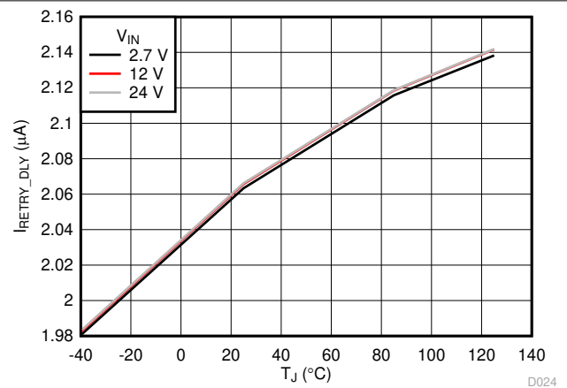
Figure 6-21. RETRY_DLY Bias Current vs Temperature
