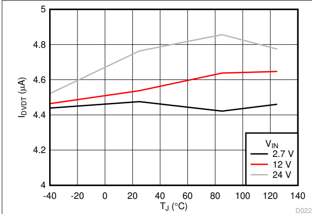
Figure 6-20. DVDT Charging Current vs Temperature
