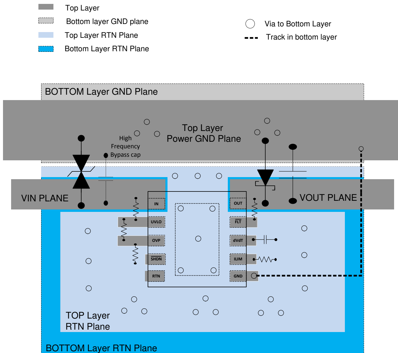
Figure 12-1. Typical PCB Layout Example With a 2 Layer PCB
