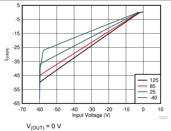
Figure 7-10. Input Supply Current vs Reverse Supply Voltage, -V_{(IN)}
