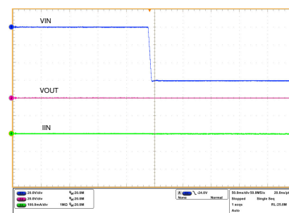
Reverse Input Polarity Protection at –60-V Supply
