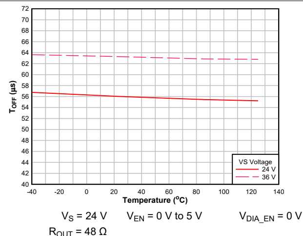
Figure 7-6. Turn-off Time ( t_{OFF} ) vs Temperature
