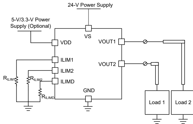
Figure 9-2. Current Limit Set Functionality
