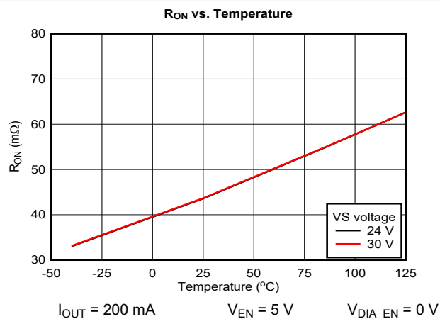
Figure 7-4. On Resistance ( R_{ON} ) vs Temperature
