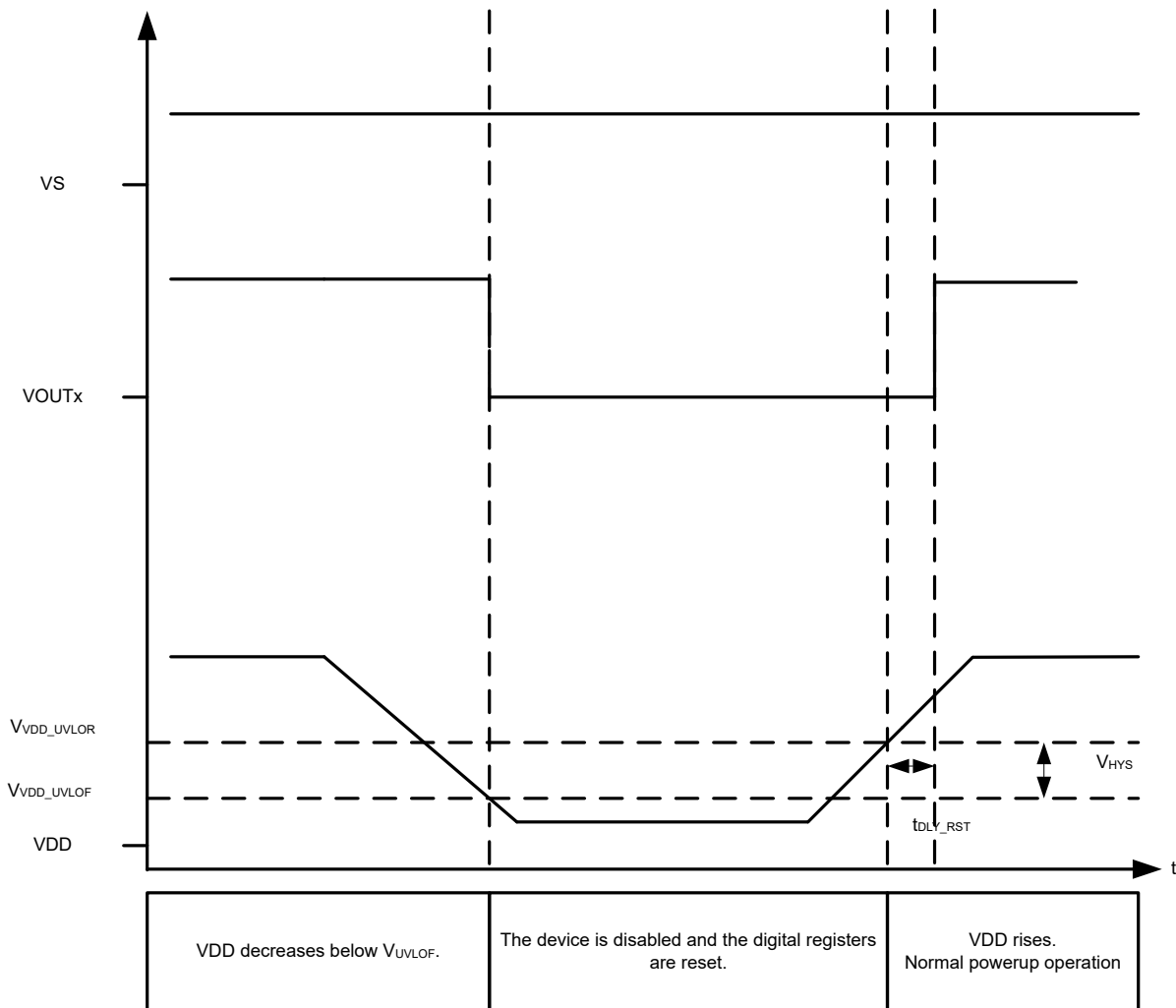
Figure 8-14. VDD UVLO
