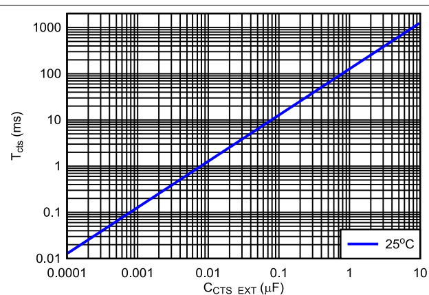
Figure 7-23. T_{CTS} vs C_{CTS}
