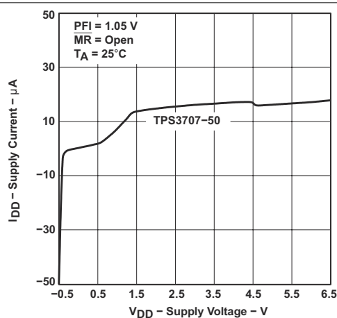
Figure 7-3. Supply Current vs Supply Voltage
