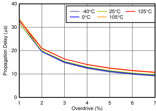
Figure 6-16. Propagation Delay vs Overdrive
