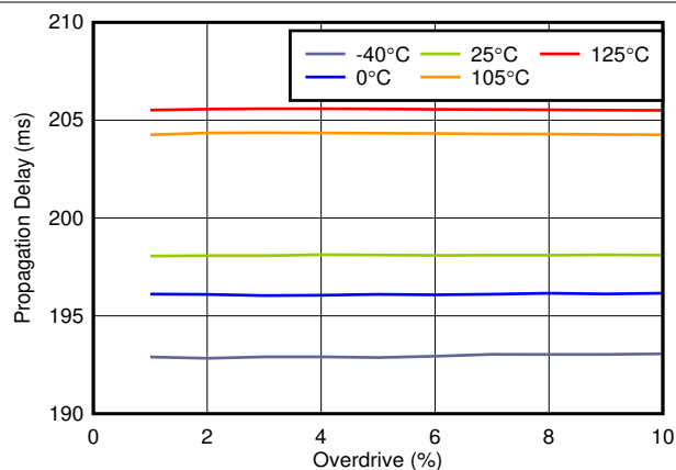
Figure 5-16. Propagation Delay vs Overdrive
