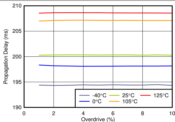
Figure 5-15. Propagation Delay vs Overdrive
