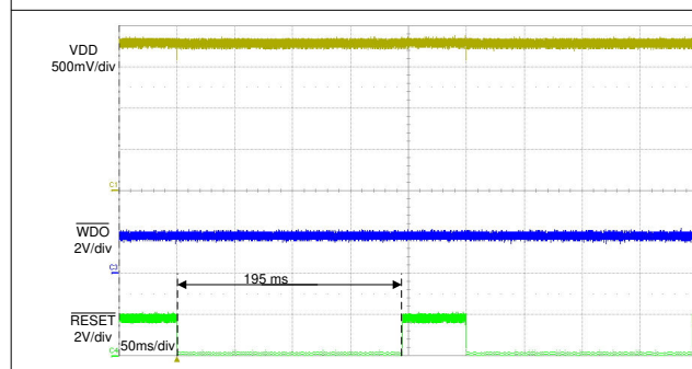
Figure 7-7. Typical RESET Delay
