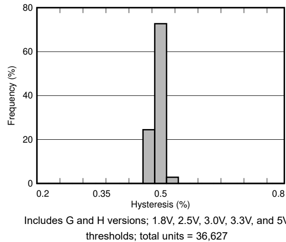
Figure 5-12. Hysteresis Histogram
