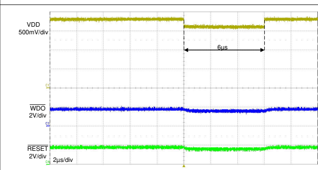
Figure 7-8. High-to-Low Glitch Immunity
