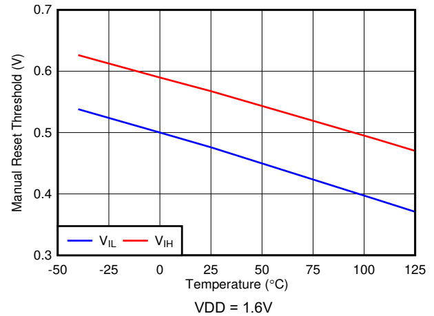
Figure 5-4. \overline{\text{MR}} Threshold vs Temperature
