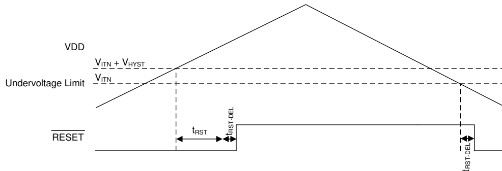
Figure 6-1. Undervoltage Detection
