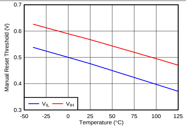
Figure 4. \overline{MR} Threshold vs Temperature
