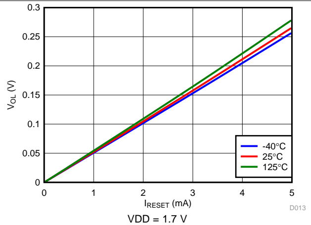
Figure 10. Low-Level Output Voltage vs RESET current
