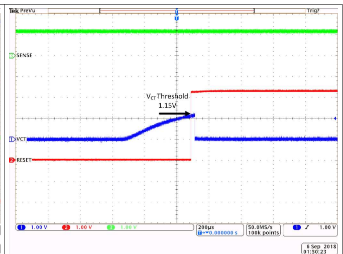
Figure 27. TPS3870-Q1 CT Bias Unlatch Function
