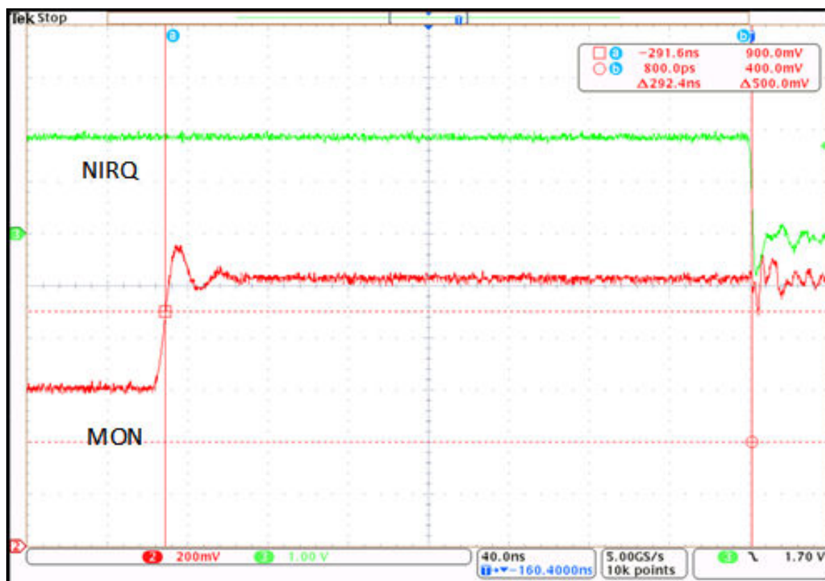
Figure 9-8. NIRQ Propagation Delay Resulting from Overvoltage Fault
