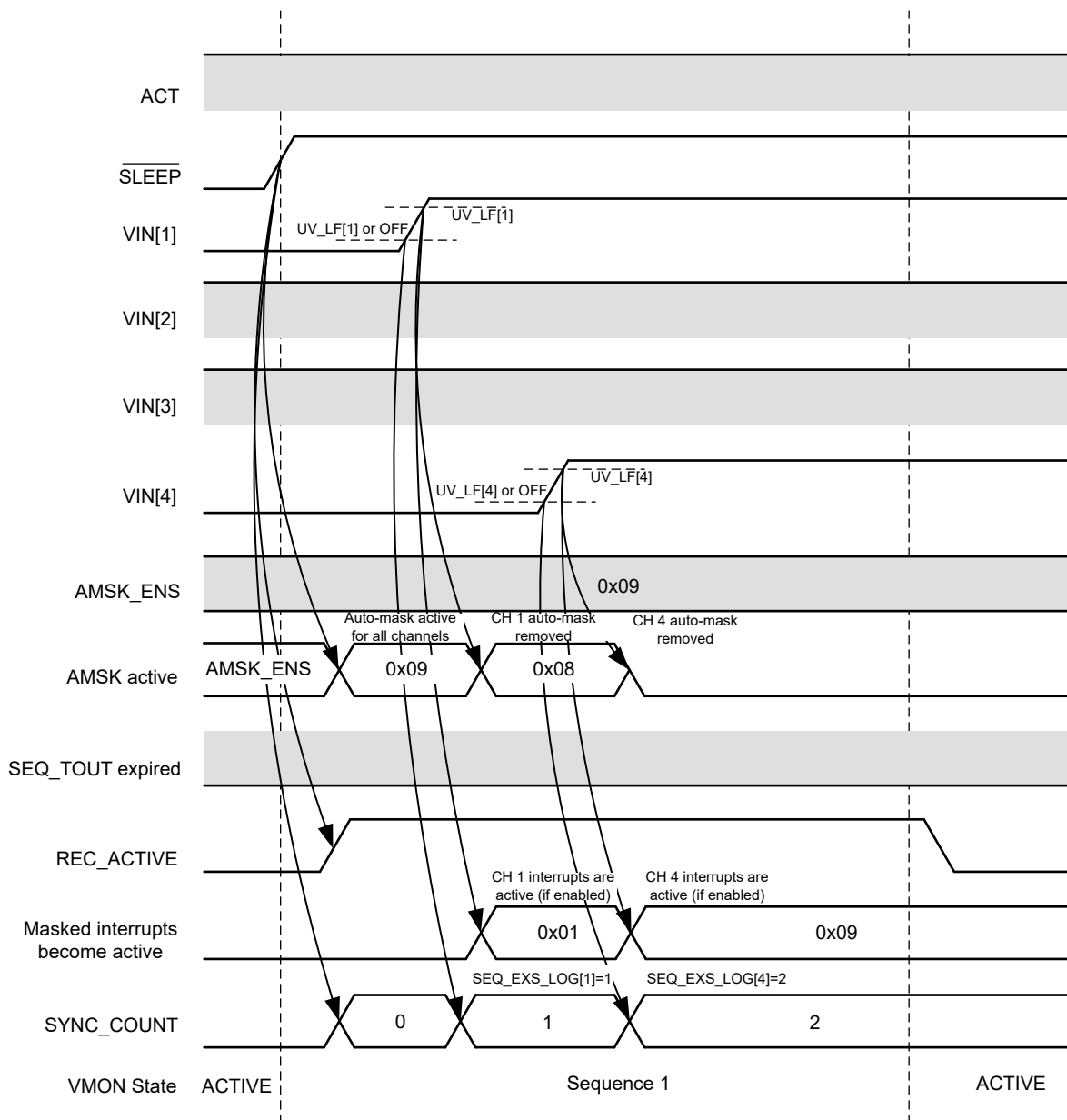
Figure 8-10. SLEEP 0→1 Transition
