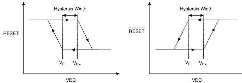
Figure 7-1. Hysteresis Diagram
