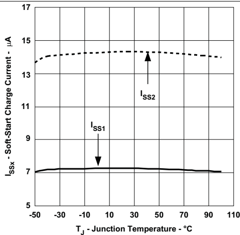
Figure 7. Soft-Start Charge Current vs Junction Temperature
