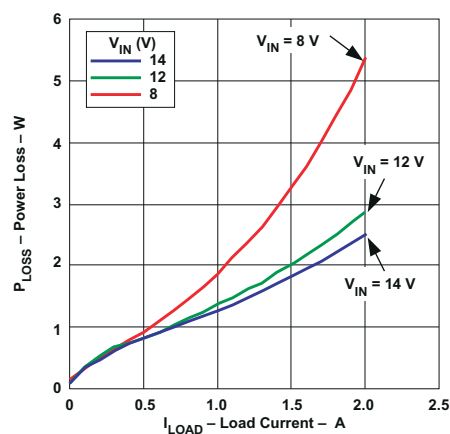
Figure 8-5. Power Loss vs Load Current
