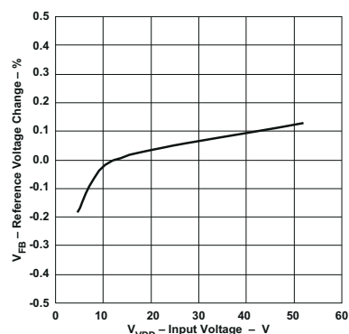
Figure 6-6. Reference Voltage Change vs Input Voltage
