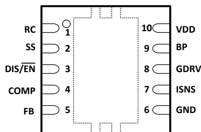
Figure 5-2. DRC 10-Pin Top View
