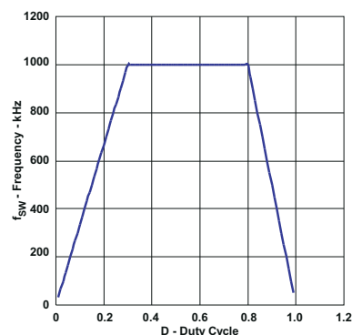
Figure 6-2. Switching Frequency vs Duty Cycle
