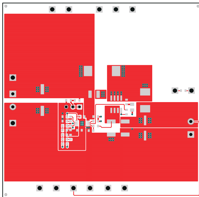
Figure 10-2. Top Copper
