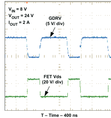
Figure 8-3. FET VDS and VGS Voltages vs Time
