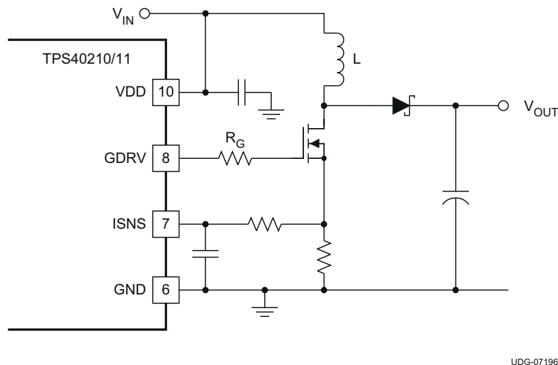
Figure 7-9. Gate Drive Resistor
