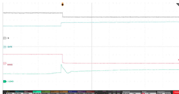
Figure 9-4. Zoom-In View of State Transition From LPM to Active Mode ( \overline{\text{LPM}} = Low, V_{\text{IN}} = 48V, \text{EN}/\text{UVLO} = High)
