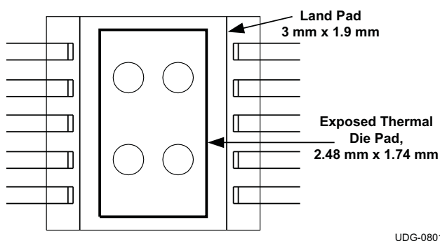
Figure 31. Recommended Land Pad Pattern
