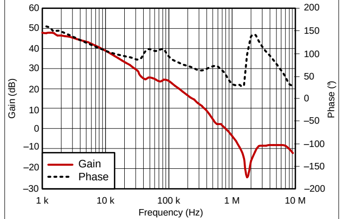
Figure 15. Bode Plot
