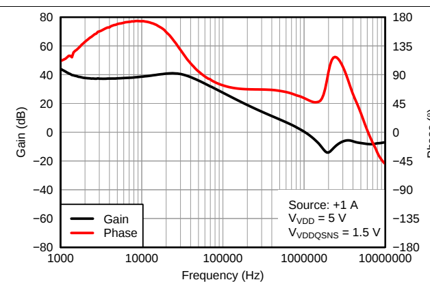
Figure 18. VTT (Source: +1 A) Bode Plot (0.75 V)
