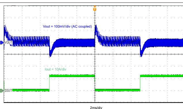
Figure 7-17. Transient Response, 0A to 12A, Slew Rate = 1.6A/μs
