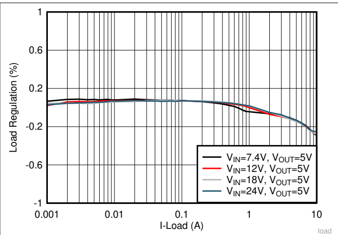
Figure 8-3. Load Regulation
