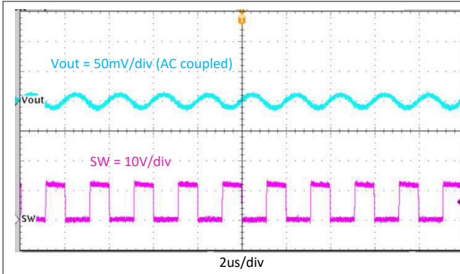
Figure 8-14. Output Voltage Ripple, I OUT = 10 A
