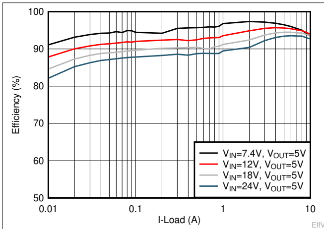
Figure 8-2. Efficiency Curve
