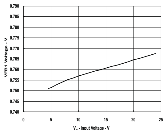
Figure 8. VFB1 Voltage vs Input Voltage
