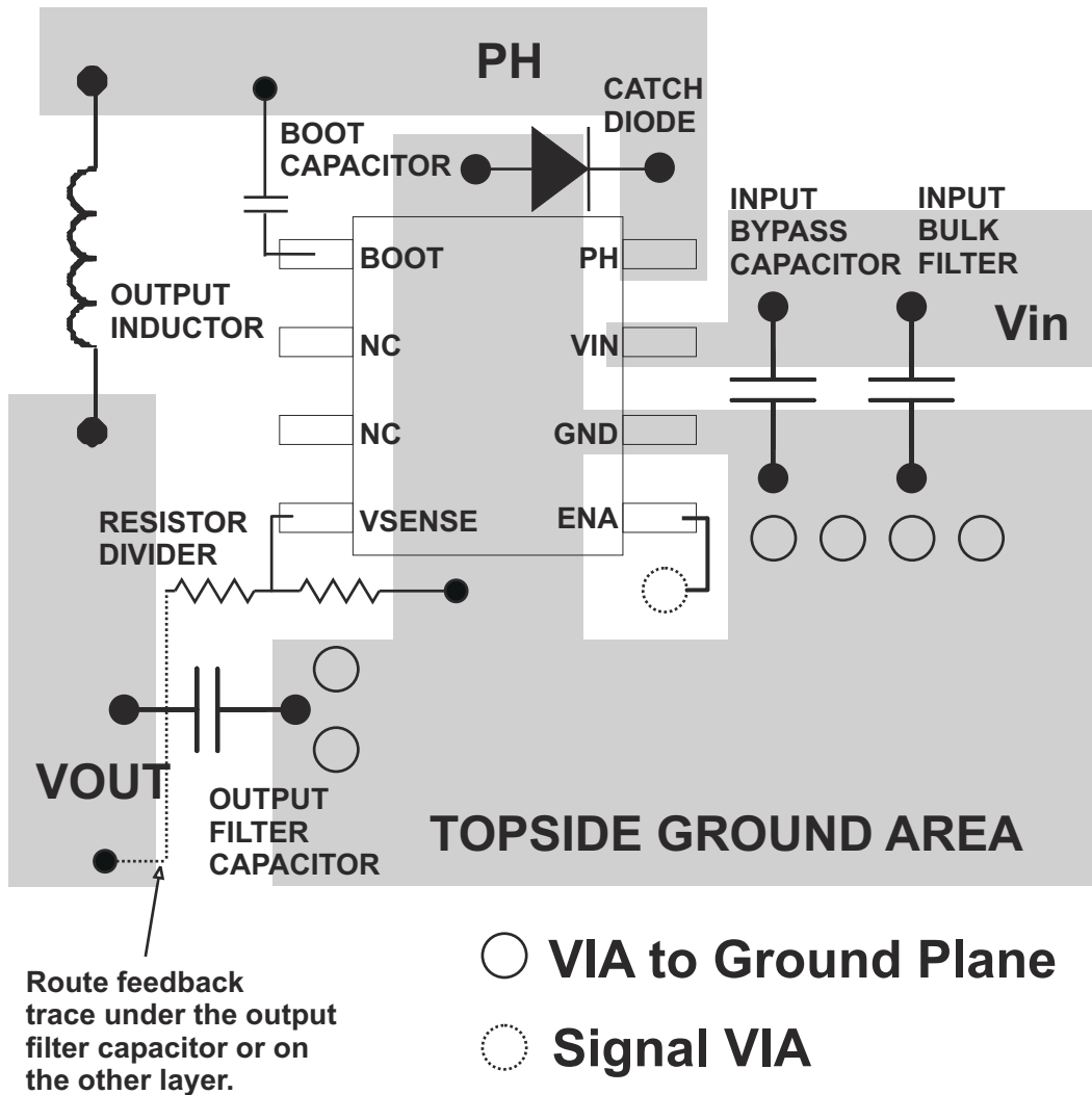
Figure 7-17. Design Layout
