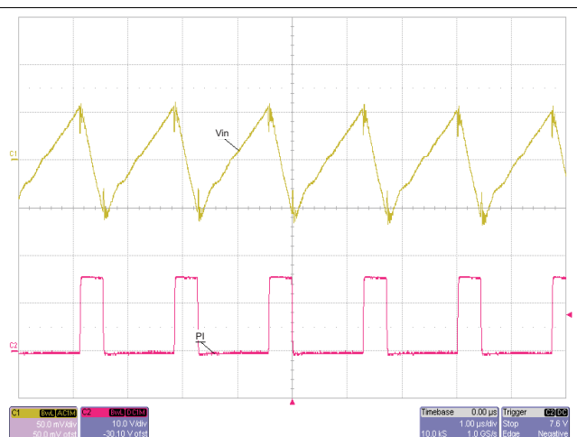
Figure 18. Input Ripple
