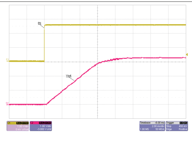
Figure 20. Startup Relative to Enable
