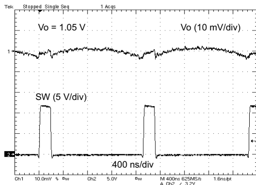
Figure 13. VOLTAGE RIPPLE AT OUTPUT ( I_O = 2\text{ A} )
